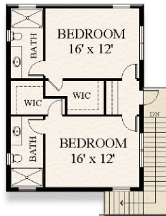
NORTHWEST GUEST HOUSE SECOND FLOOR
